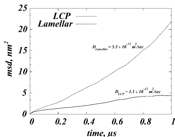
Figure 8. Mean-square-displacement ( msd ) as a function of time calculated for rhodopsin in the 9.9 MAG lipid cubic phase (LCP) and in the 9.9 MAG lamellar membrane (Lamellar). Corresponding diffusion coefficient values, calculated from the linear fit performed in [0 \mu\text{s}; 1 \mu\text{s}] time interval, are D_{LCP} = 1.1 \times 10^{-12} \text{ m}^2/\text{sec} and D_{LAMELLAR} = 5.5 \times 10^{-12} \text{ m}^2/\text{sec} .
